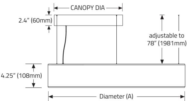
SS3 VERTICAL - INTEGRAL DRIVER
