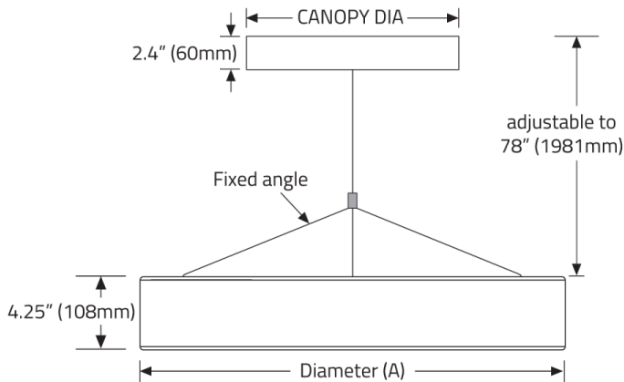
SS4 HUB - INTEGRAL DRIVER
