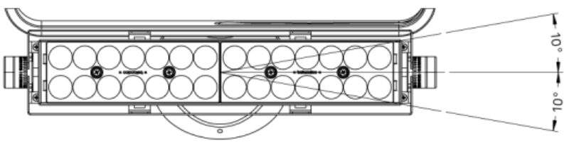
VIEW NORMAL TO YOKE
